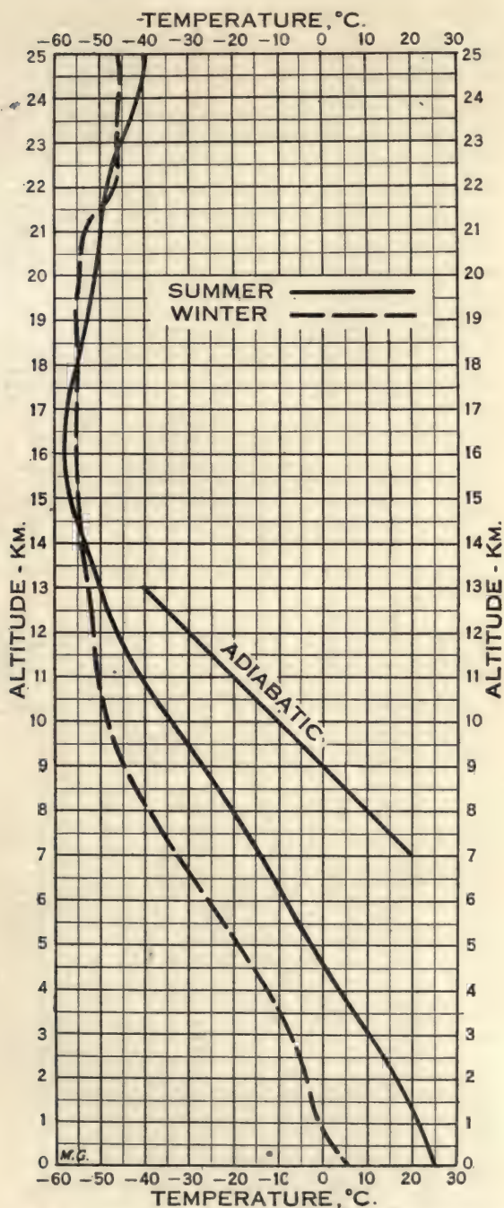
FIGURE 28. Mean summer and winter free air temperature gradients, °C, from sounding balloon records in the Central and Western States.
